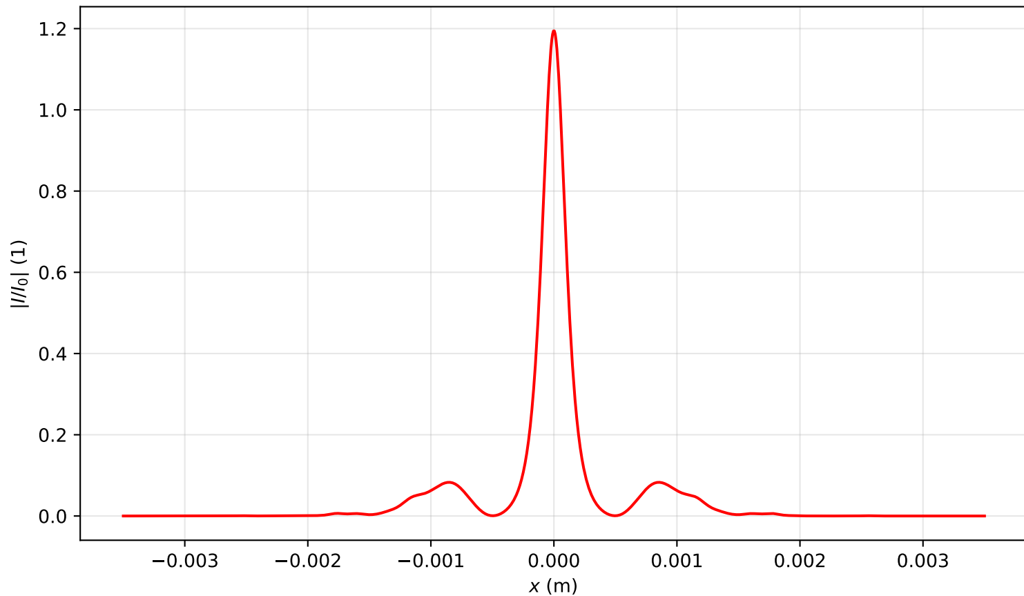
Intensity profile I(x, y = 0, z = 1.911)/I_0 , \text{Pin}=9.0\text{Pcr} , artificial time
